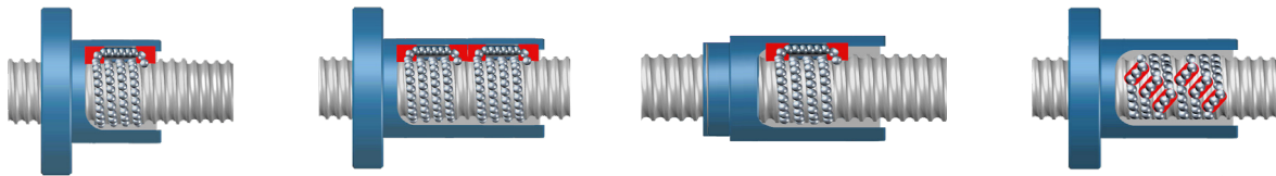
*Nut A: Single Nut Recirculating *Nut B: PitchShift Nut C: Nose Thread *Nut D: Single Nut Insert Transfer
